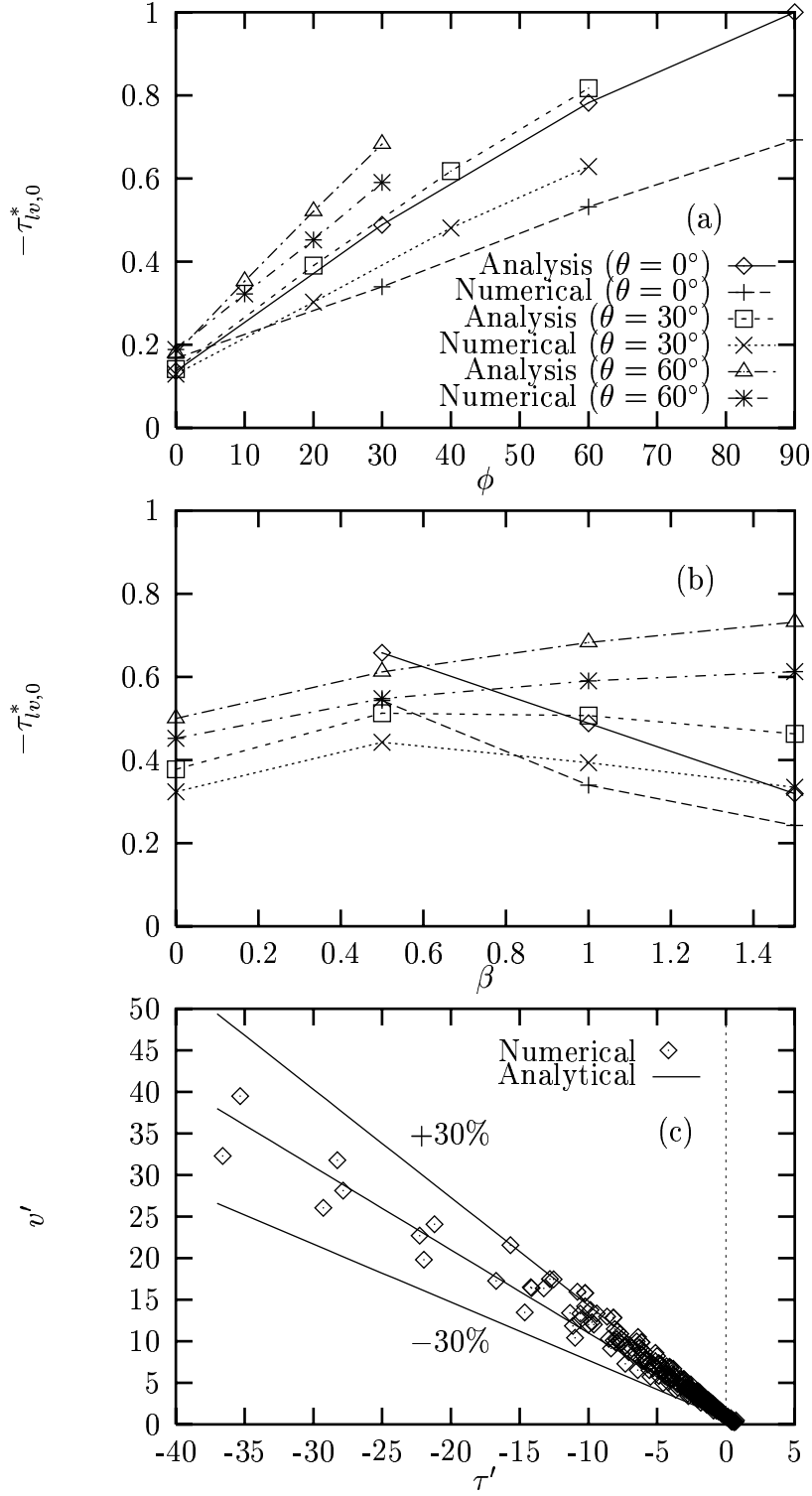
Figure 10: Numerical and semi-analytical solution comparison: (a) -\tau_{lv,0}^* versus \phi for \beta = 1.0 (from Fig. 3); (b) -\tau_{lv,0}^* versus \beta for \phi = 30^\circ (from Fig. 6); (c) Normalized mean velocity versus normalized shear stress at the liquid-vapor interface (from Figs. 3 and 6).
