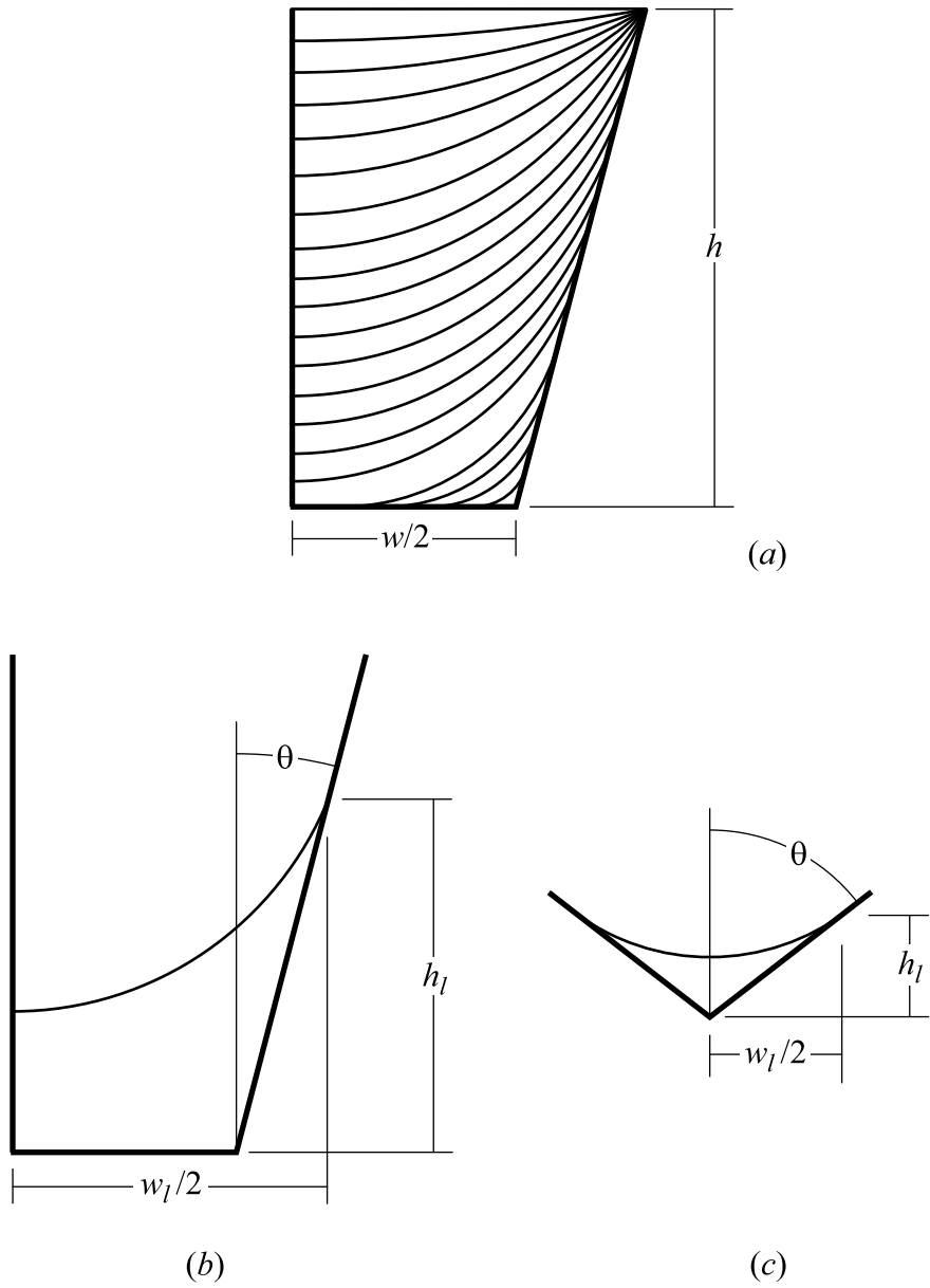
Figure 11: Effect of groove fill ratio on liquid flowing in a trapezoidal groove: (a) Parametric analysis (to scale, h = 0.03831 cm, w = 0.03445 cm, \theta = 14.62^\circ ); (b) Definition of variables prior to bifurcation of the liquid; (c) Definition of variables after bifurcation of the liquid.
