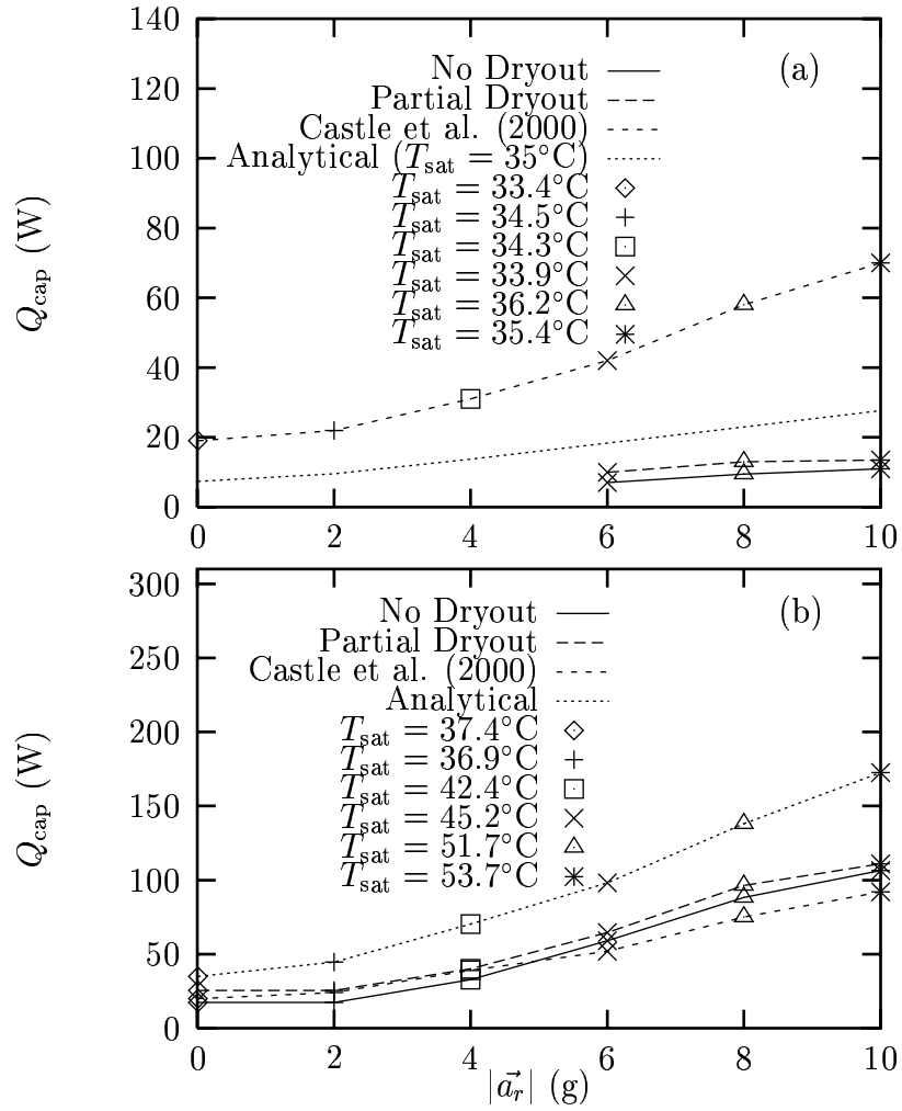
Figure 15: Maximum heat transport versus radial acceleration: (a) A_i/A_g = 0.5 ; (b) A_i/A_g = 1.0 .
