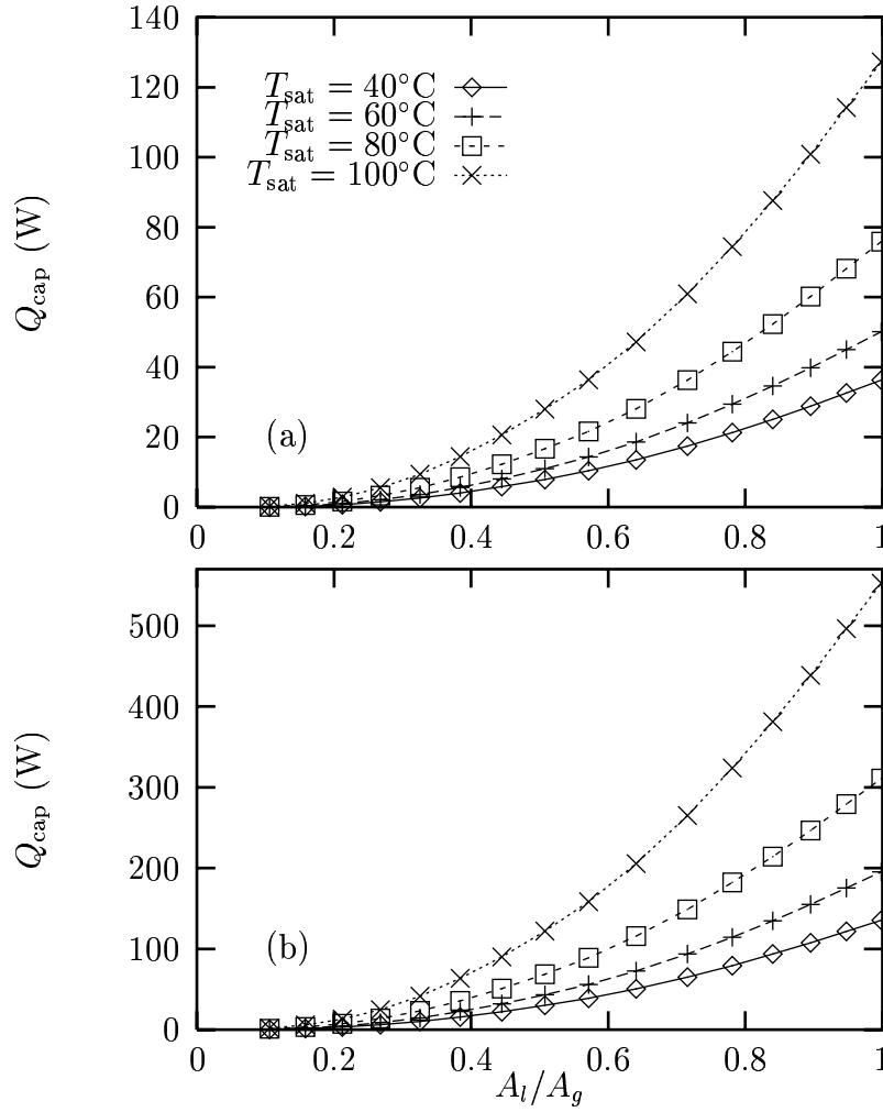
Figure 14: Maximum heat transport versus groove fill ratio for several working temperatures (Ethanol): (a) |\vec{a}_r| = 0.0\text{-g} ; (b) |\vec{a}_r| = 10.0\text{-g} .
