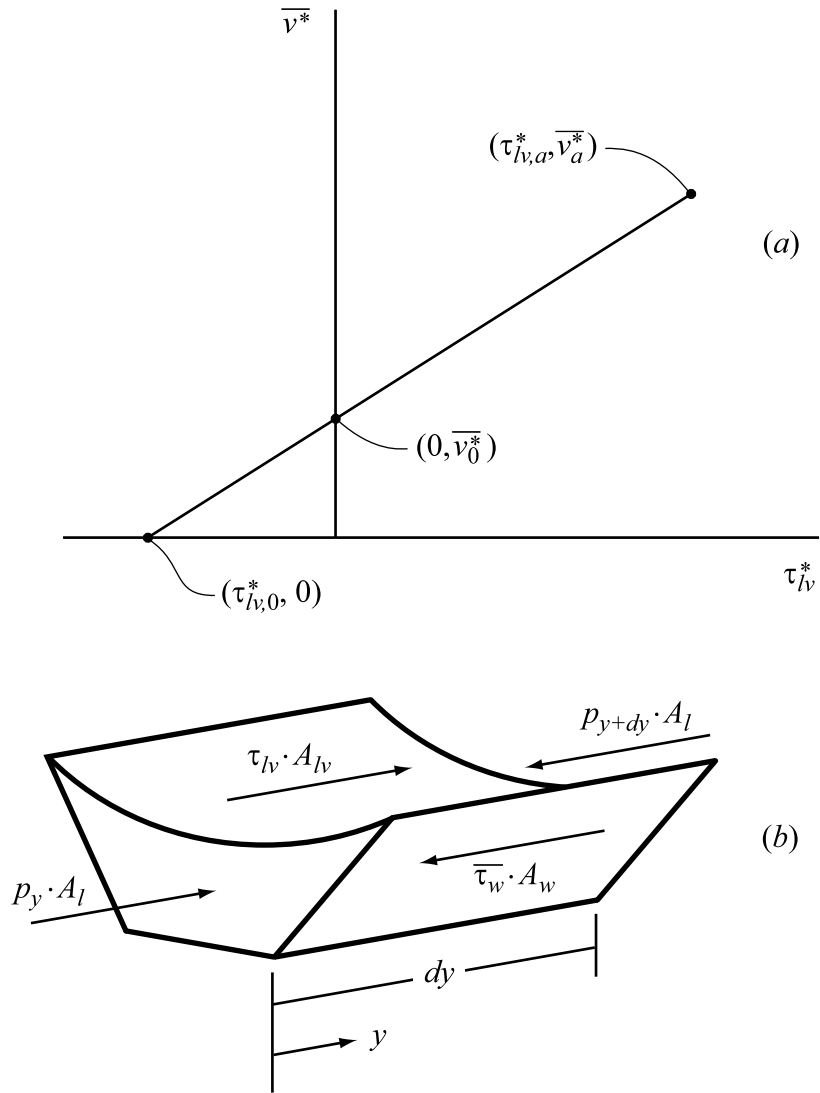
Figure 9: Semi-analytical and two-point numerical solutions for \bar{v}^* : (a) Definition of parameters; (b) Force balance on the liquid in a trapezoidal groove.
