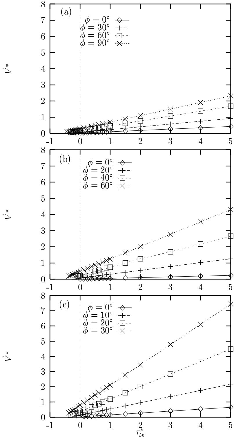
Figure 5: \dot{V}^* versus \tau_{lv}^* for laminar flow in trapezoidal grooves ( \beta = 1.0 ): (a) \theta = 0^\circ ; (b) \theta = 30^\circ ; (c) \theta = 60^\circ .
