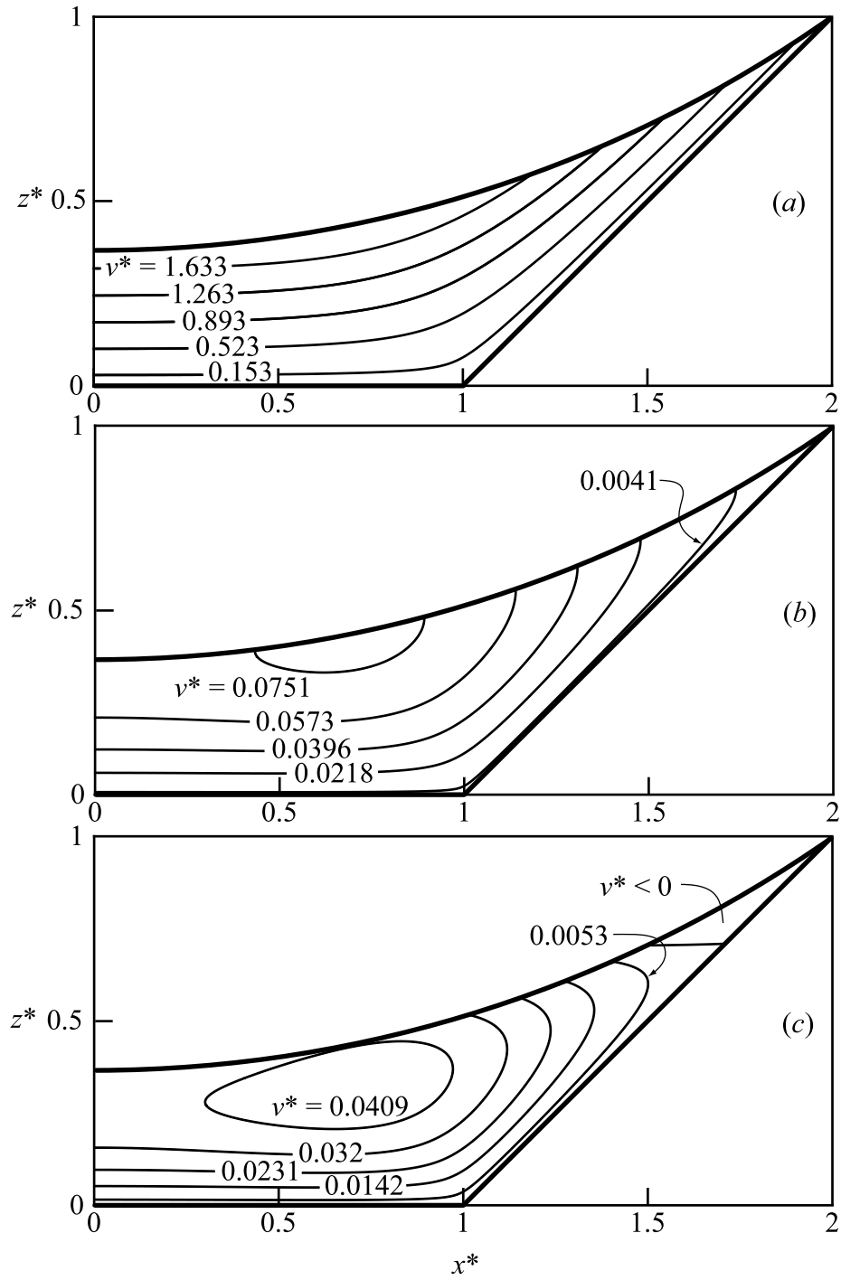
Figure 2: Dimensionless velocity fields for laminar flow in trapezoidal grooves ( \beta = 1.0 , \phi = 10^\circ , \theta = 45^\circ ): (a) \tau_{lv}^* = 5.0 (cocurrent flow); (b) \tau_{lv}^* = 0.0 ; (c) \tau_{lv}^* = -0.1 (countercurrent flow).
