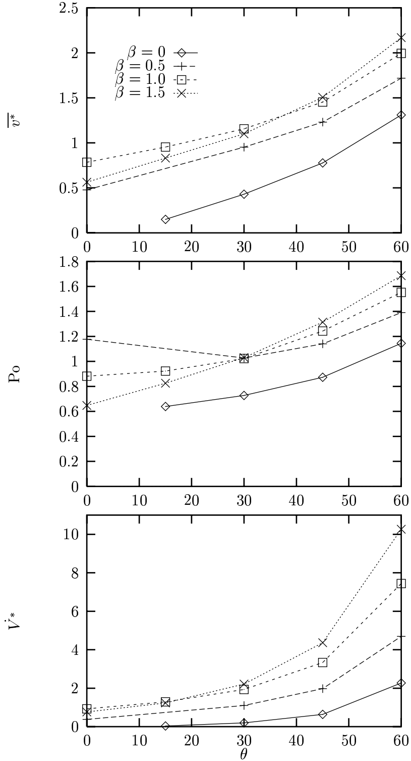
Figure 7: \overline{v^*} , Po and \dot{V}^* versus \theta for laminar flow in trapezoidal grooves ( \phi = 30^\circ , \tau_{lw}^* = 5.0 ).
