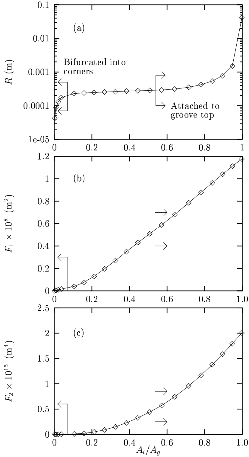
Figure 12: Effect of groove fill ratio: (a) Radius of curvature of the liquid-vapor interface; (b) Mean velocity parameter; (c) Volumetric flow rate parameter.
