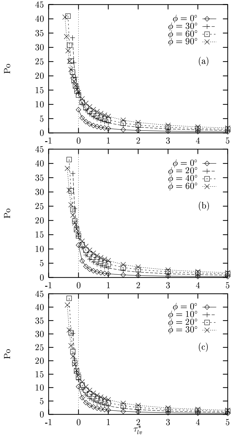
Figure 4: P_o versus \tau_{lv}^* for laminar flow in trapezoidal grooves ( \beta = 1.0 ): (a) \theta = 0^\circ ; (b) \theta = 30^\circ ; (c) \theta = 60^\circ .
