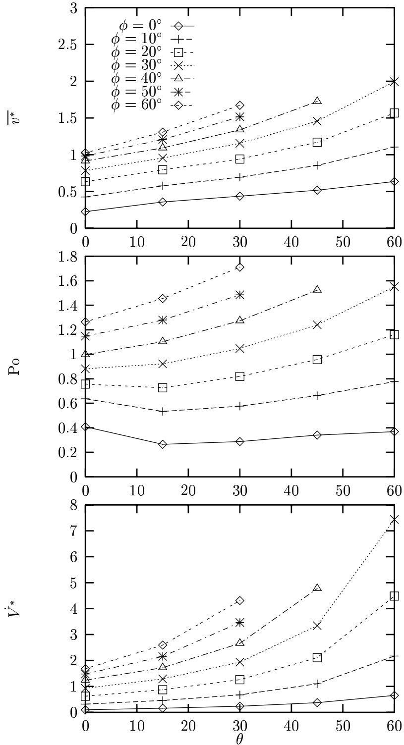
Figure 8: \bar{v}^* , P_o and \dot{V}^* versus \theta for laminar flow in trapezoidal grooves ( \beta = 1.0 , \tau_{lw}^* = 5.0 ).
