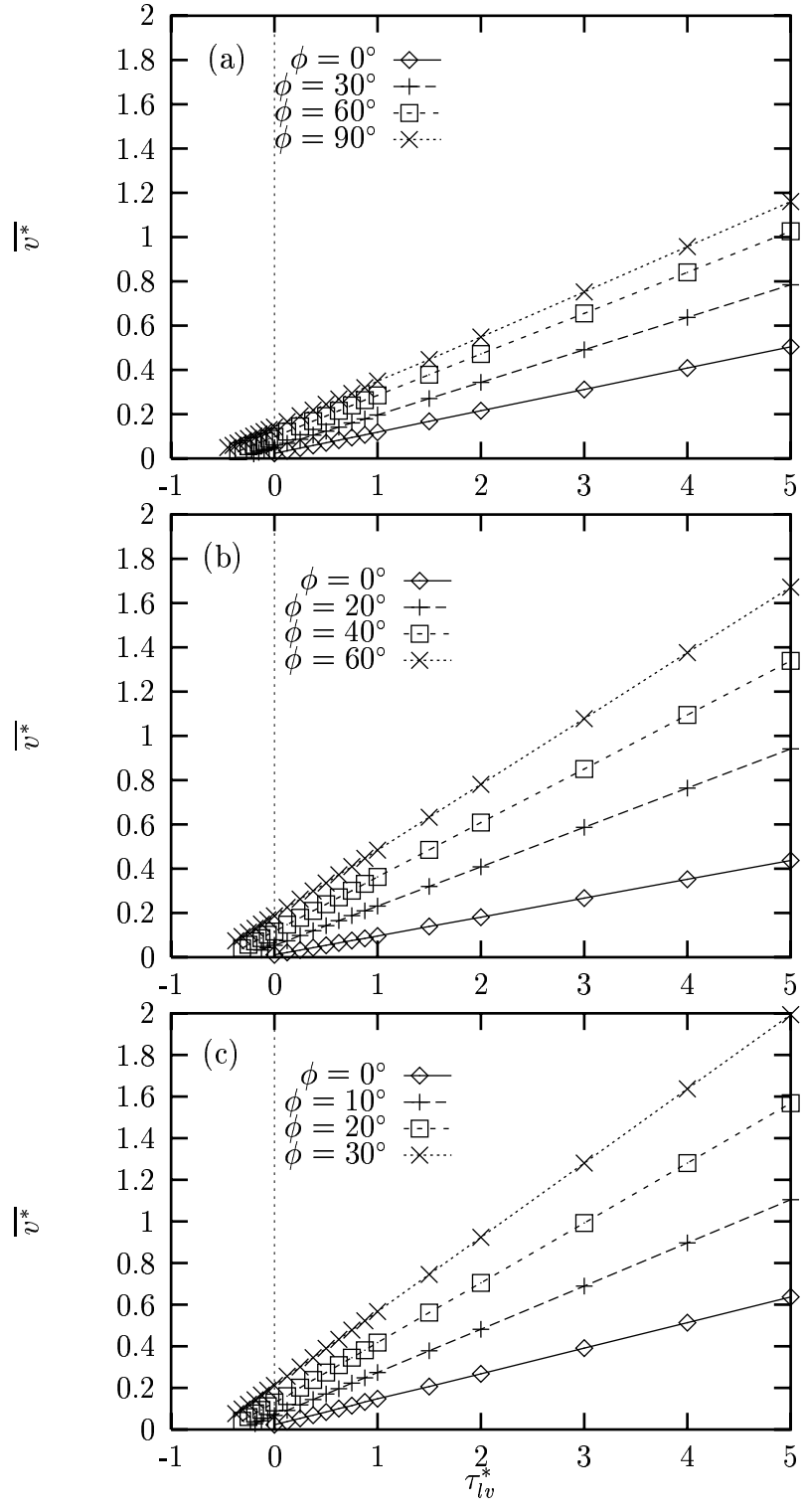
Figure 3: \overline{v}^* versus \tau_{lv}^* for laminar flow in trapezoidal grooves ( \beta = 1.0 ): (a) \theta = 0^\circ ; (b) \theta = 30^\circ ; (c) \theta = 60^\circ .
