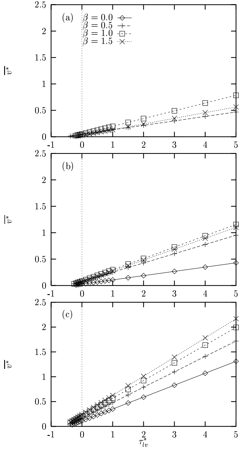
Figure 6: \overline{v}^* versus \tau_{lv}^* for laminar flow in trapezoidal grooves ( \phi = 30^\circ ): (a) \theta = 0^\circ ; (b) \theta = 30^\circ ; (c) \theta = 60^\circ .
