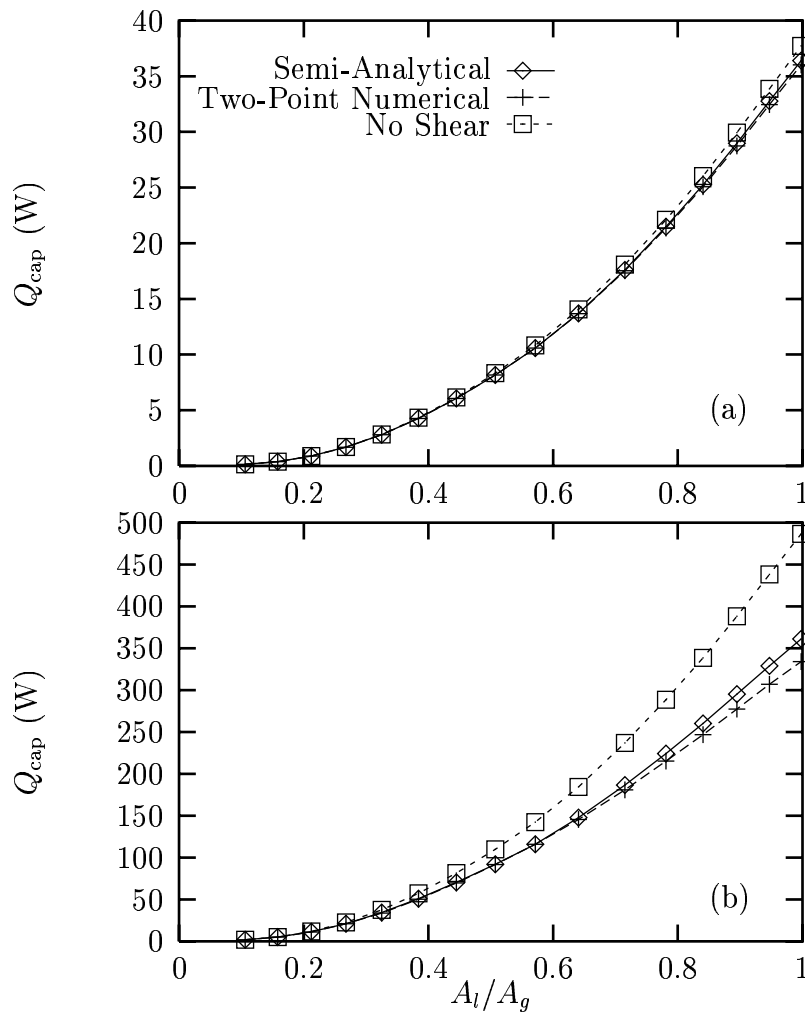
Figure 13: Maximum heat transport predicted by the closed-form solution versus groove fill ratio (Straight axial grooves, no body forces, T_{\text{sat}} = 40^\circ\text{C} ): (a) Ethanol; (b) Water.
