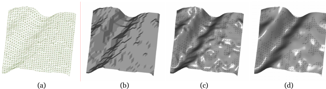
Fig. 4. (a) Triangulation of a digital elevation map. This data set is courtesy of USGS. (b) The triangle mesh in shaded form. (c) Approximation of the mesh by the proposed approximation using the mesh edges as the 3-D lines. (d) A smoother approximation to the same mesh.
