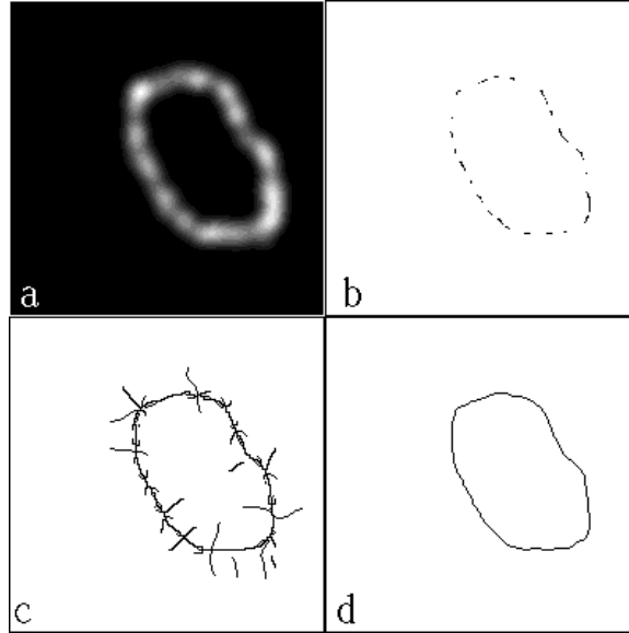
Figure 2: (a) A synthetically generated gradient image. (b) Edges obtained by the nonmaxima suppression of Canny. (c) The minor edges. (d) Edges obtained by the revised Canny edge detector.
