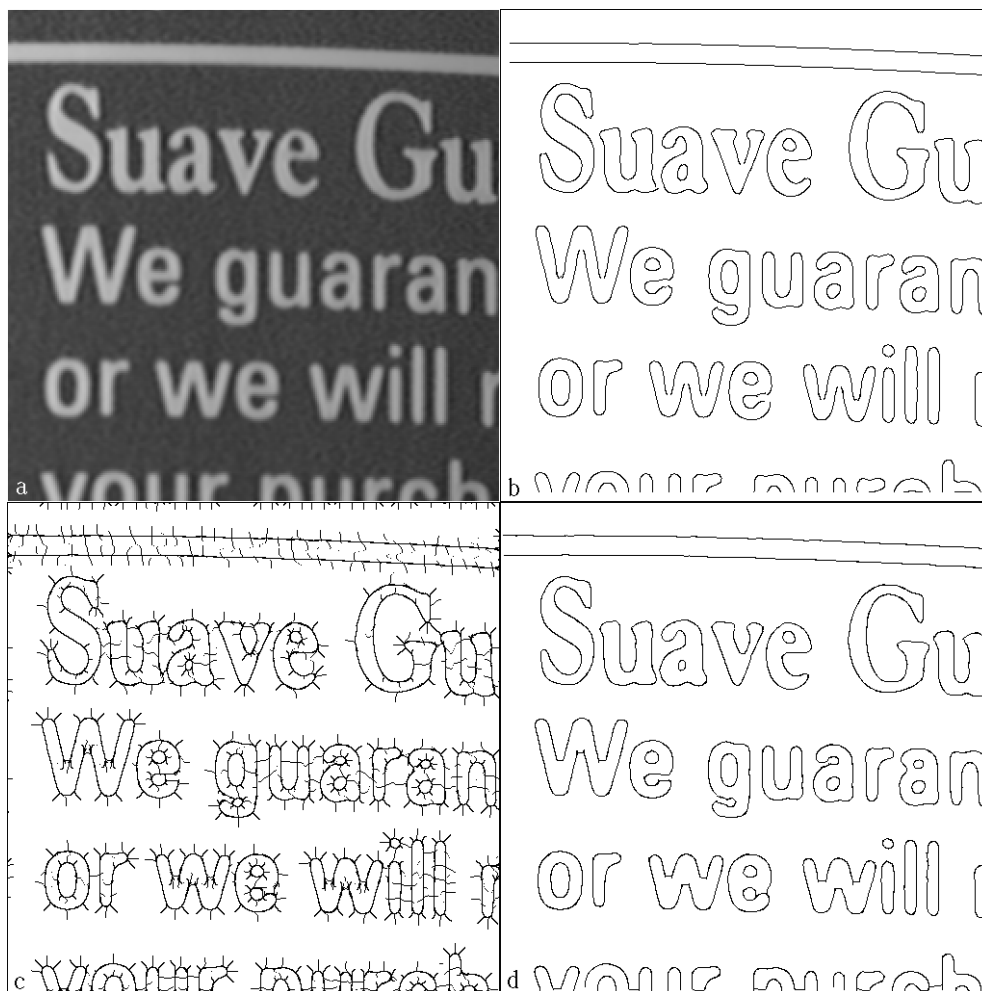
Figure 4: (a) An image of printed text. (b) Edges determined by the Canny edge detector. (c) The minor edges. (d) Edges determined by the revised Canny edge detector.
