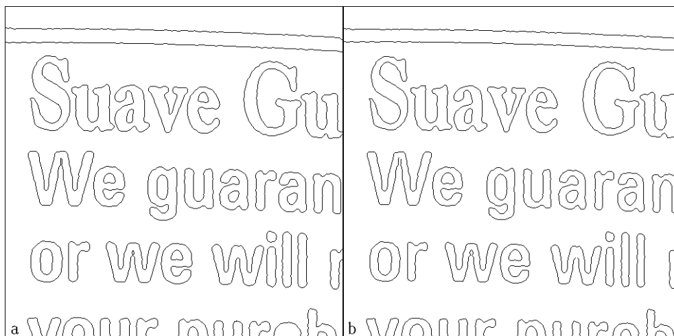
Figure 5: (a) The zero-crossings of the Laplacian of Gaussian of the printed text image after hysteresis thresholding. (b) The zero-crossing edges after removal of the phantom edges.
