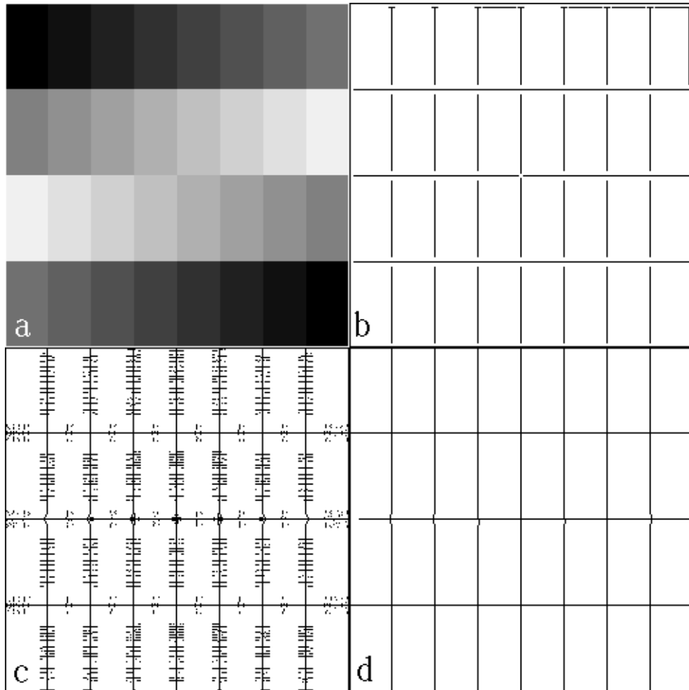
Figure 3: (a) An image with 32 homogeneous regions. (b) Edges determined by the Canny edge detector. (c) The minor edges. (d) Edges determined by the revised Canny edge detector.
